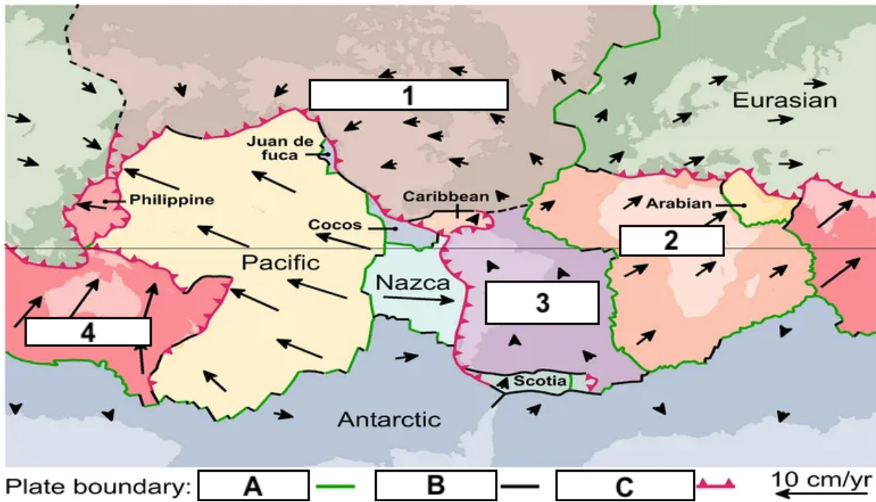
NAMED TECTONIC PLATES and their motion
